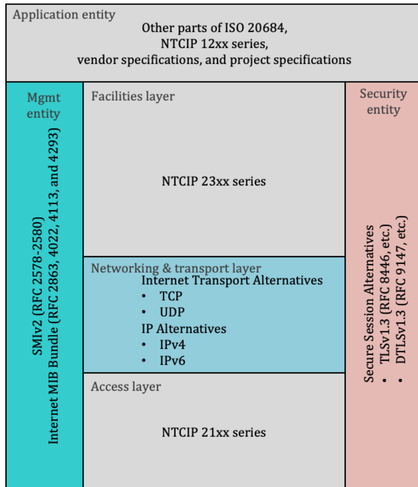
Figure 1: Internet Transport Profile Relationships
